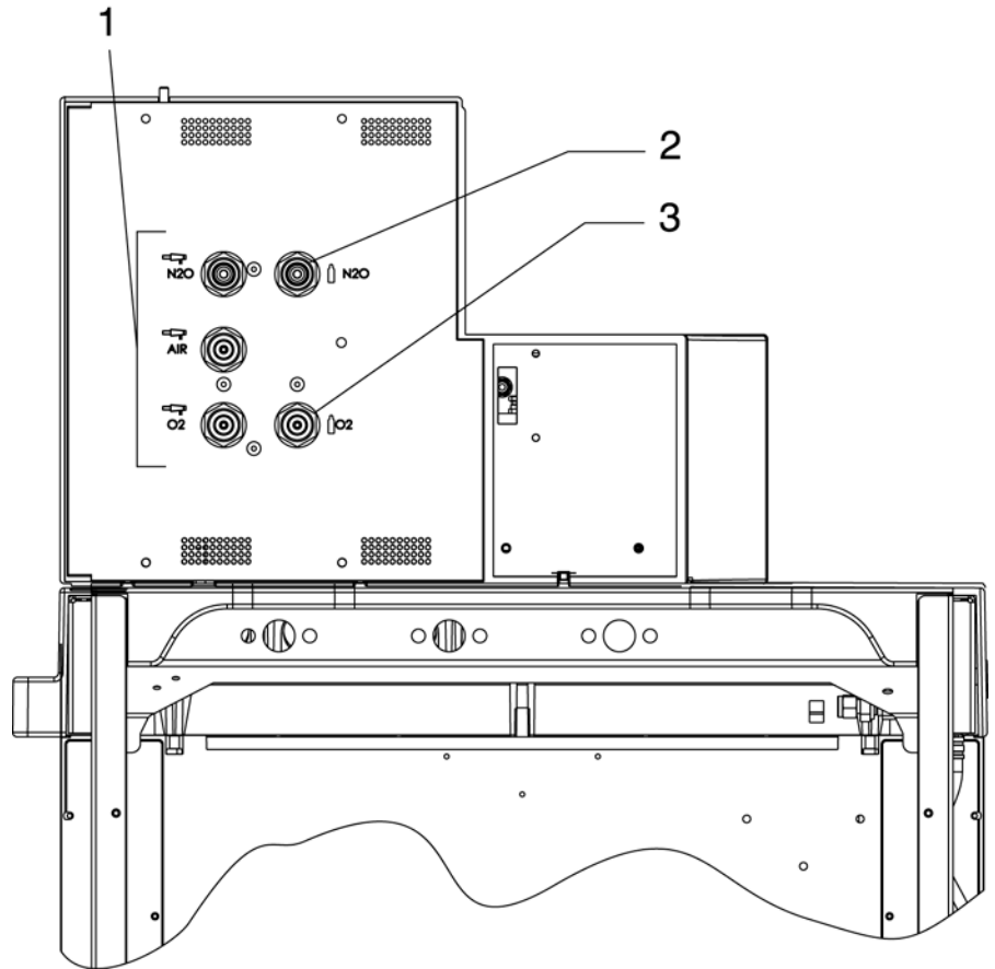
Figure 4 Rear view showing gas pipeline and cylinder connections (units without PIN index cylinder connections), for legend see Table 4
