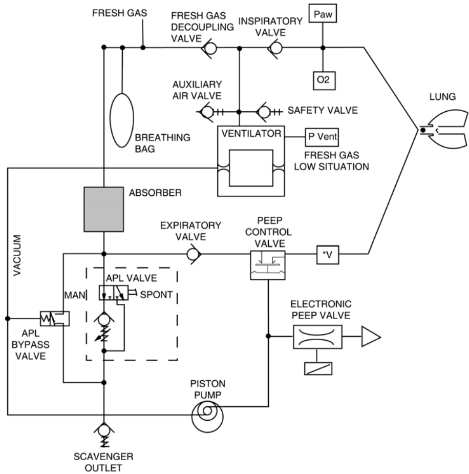
Figure 5 Function diagram of Fabius GS - Cosy 2 breathing system
