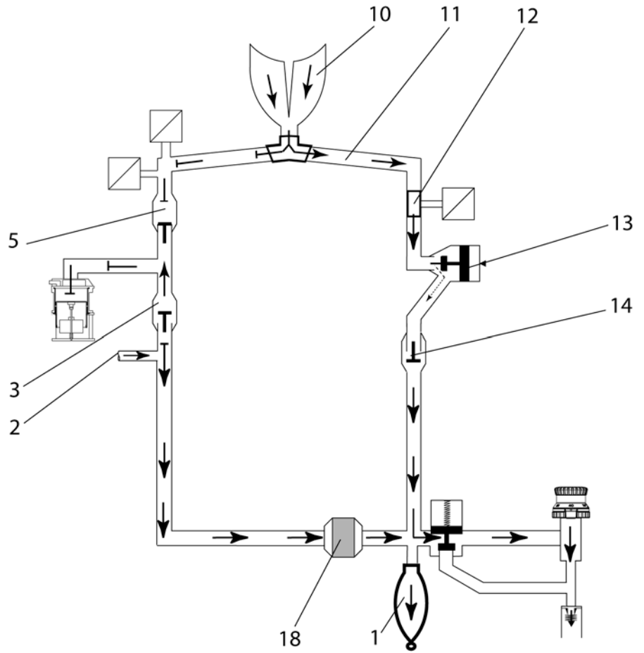
Figure 19 Manual ventilation (expiration) - Cosy 2.5 (2.6) breathing system; for legend see Table 8
