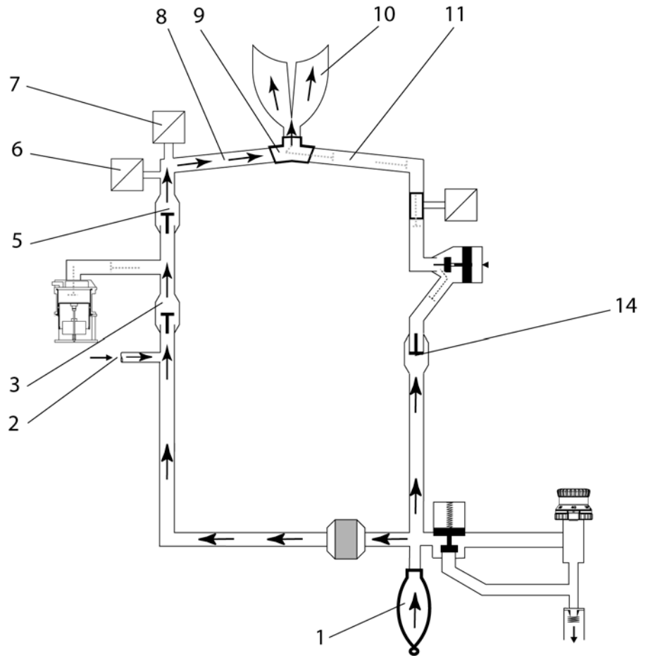
Figure 21 Spontaneous (inspiration) - Cosy 2.5 (2.6); breathing system; for legend see Table 8
