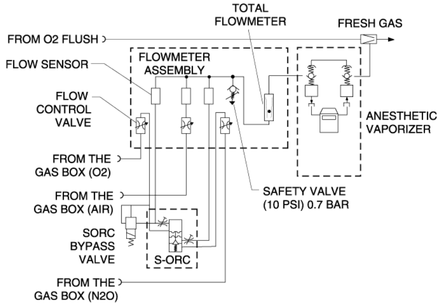
Figure 11 SORC function diagram, part 1
